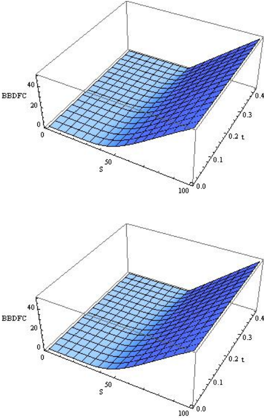
Figure 5: Approximate and exact solutions for the call option for Example 4.1, h = 1/12, \Delta S = 20 .
