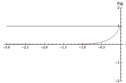
Figure 2: Plot confirming L_0 -stability
