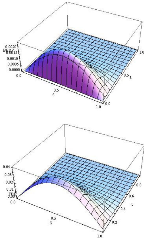
Figure 7: Approximate and exact solutions for Example 4.2, h = 1/64 , \Delta S = 1/16 .
