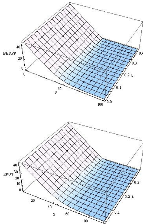
Figure 6: Approximate and exact solutions for the put option for Example 4.1, h = 1/12, \Delta S = 20 .
