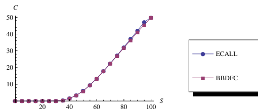
Figure 3: Call Curves for Example 1.
