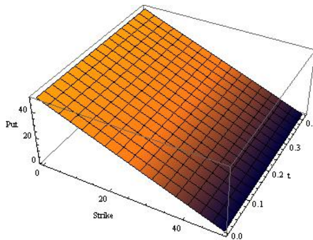
Figure 8: Put values against strike and time for Example 3.
