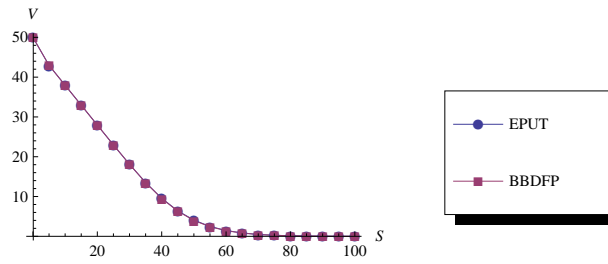
Figure 4: Put Curves for Example 1.
