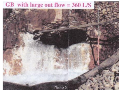
Figure 7: Spring of discharge 360l/sec which is connected to the ground water aquifer connected to the reservoir
