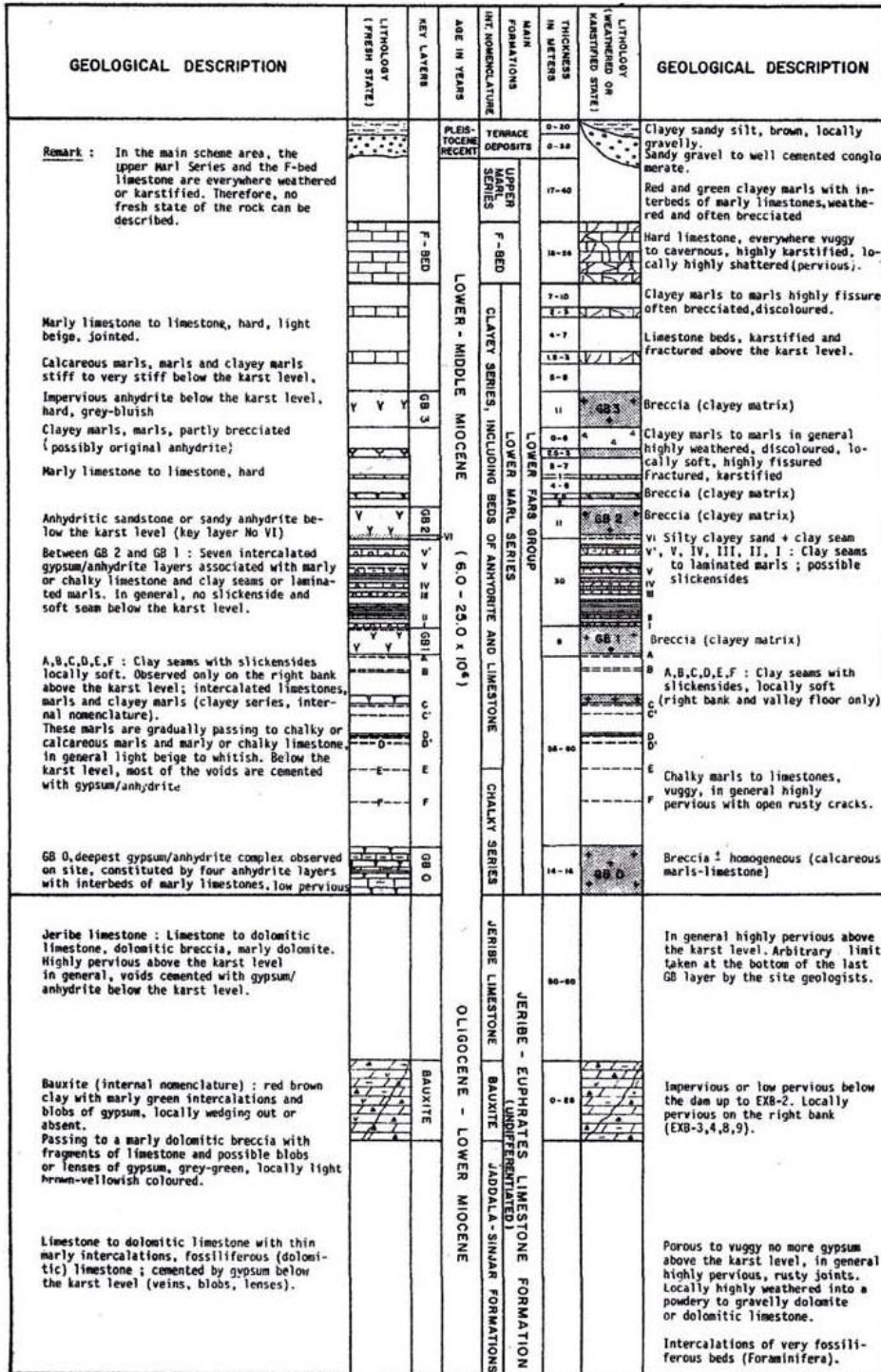
Figure 2: Lithological column of beds at Mosul Dam site [7].
