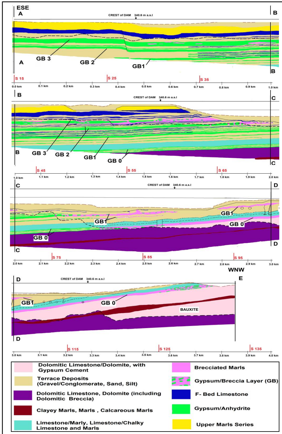
Figure 3: Geologic cross section along the axis of the dam.
