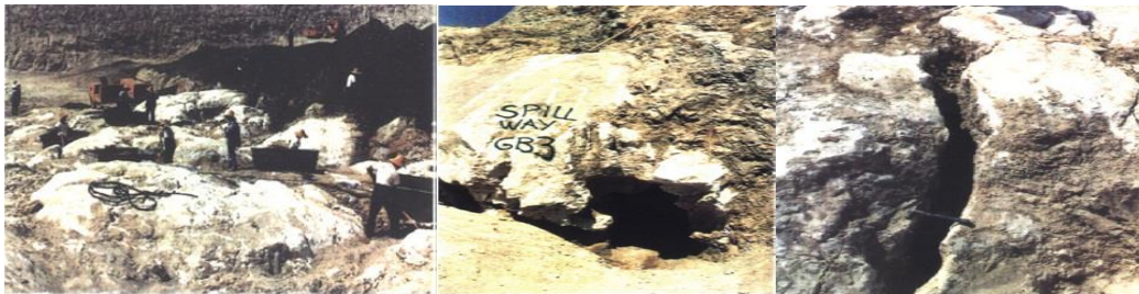
Figure 8: Karstified gypsum in the foundations of the dam (left and middle), Solution crack (right).
