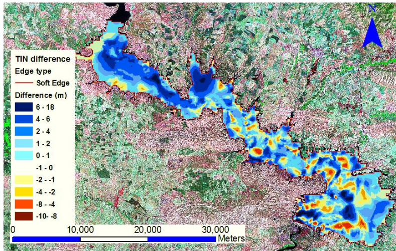
Figure 12: Holes noticed at the bed of Mosul reservoir [17].
