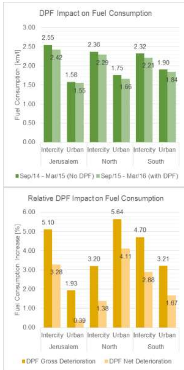
Figure 8: DPF effect on fuel consumption
