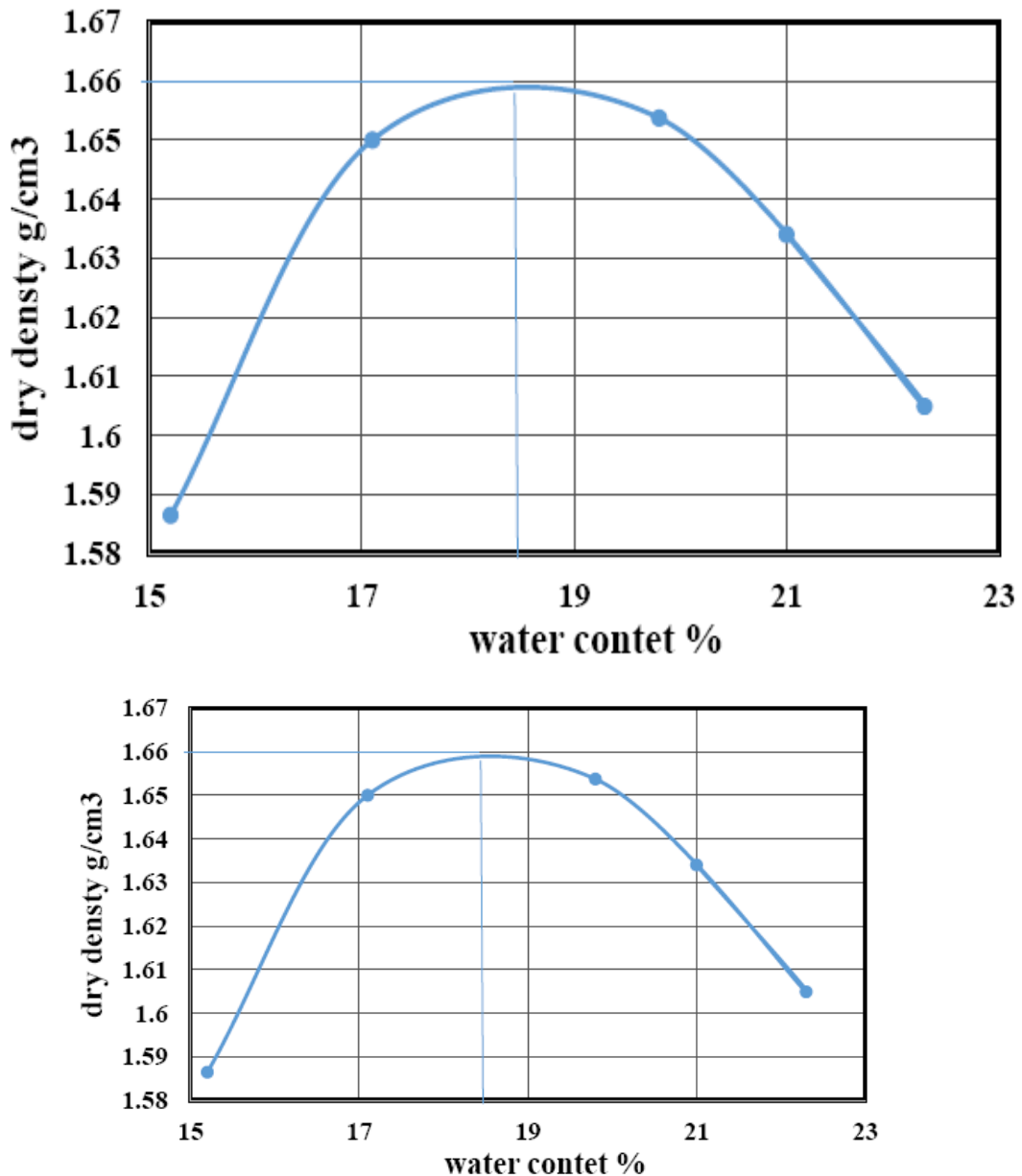
Fig. 1: Moisture-density relationship for subgrade soil used.
