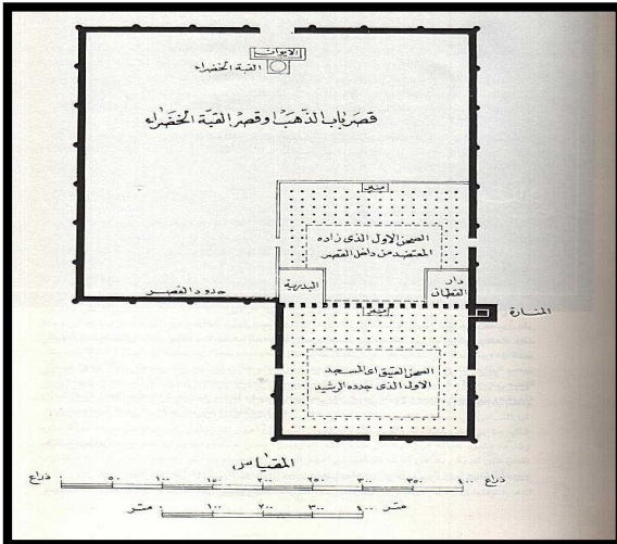
Figure 14 : Plan of Mosque and Gold
