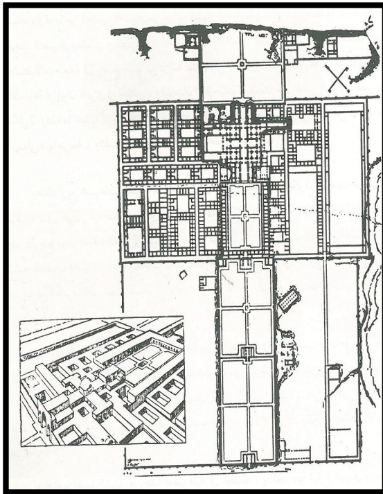
Figure 29 : Blkuar Palace planned
