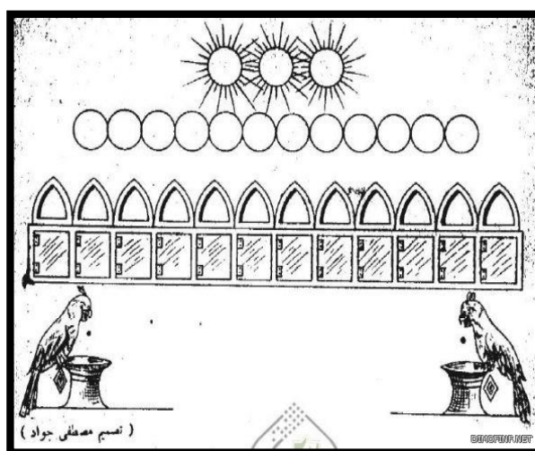
Figure 21: Plan of the Water Clock [31]
