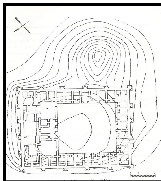
Figure 4 : Plan of Umayyad Palace in Basra [5]
