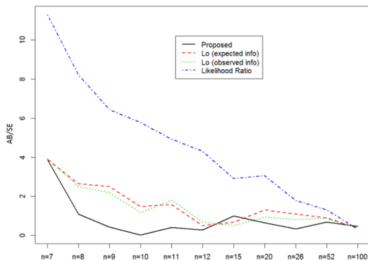
Figure 1: The Effect of Sample Size on AB/SE under AR(1) Returns (Upper graph: \rho = -0.5 ; Lower graph: \rho = 0.5 )
