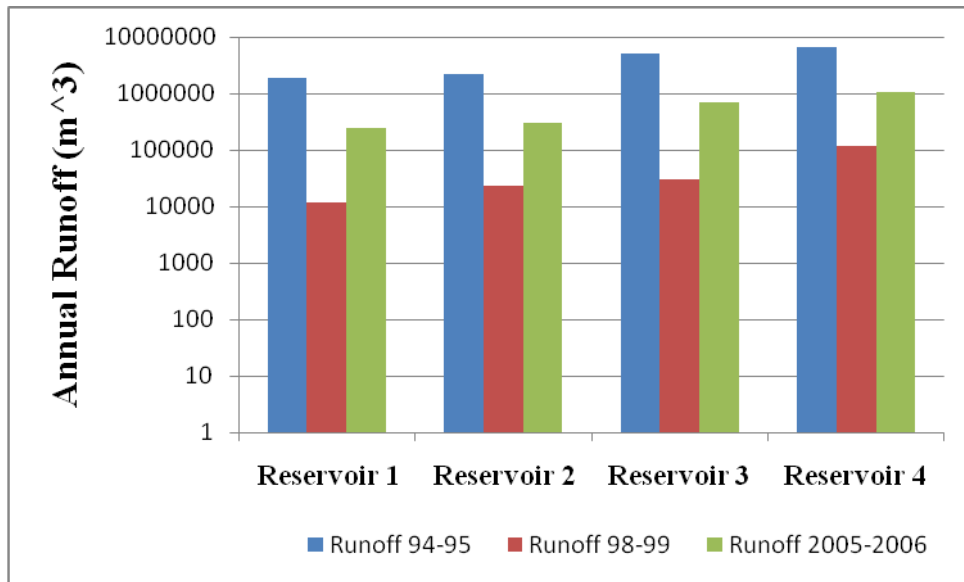
Figure 3: Annual runoff of the recorded rainfall scenarios (S1, S2 and S3)
