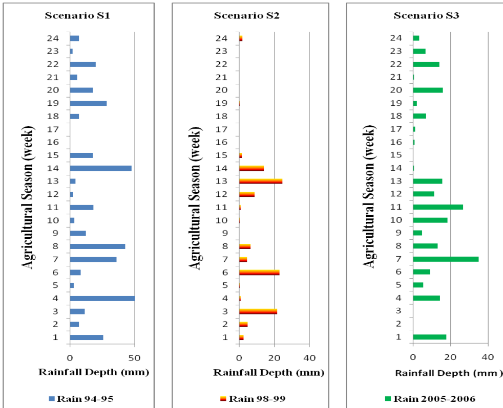
Figure 2: Rainfall Events through three selected weekly recorded rainfall Scenarios (S1, S2 and S3)
