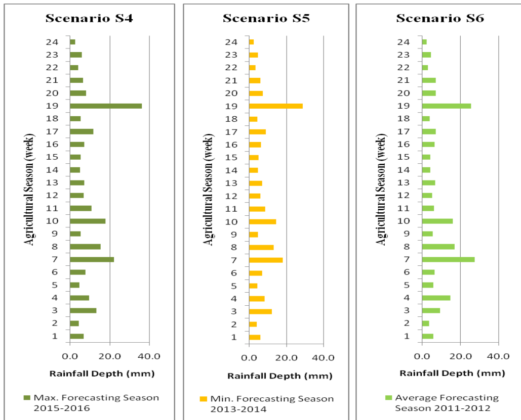
Figure 7: Rainfall events through three diagnosed weekly forecasting rainfall Scenarios (S4, S5 and S6).
