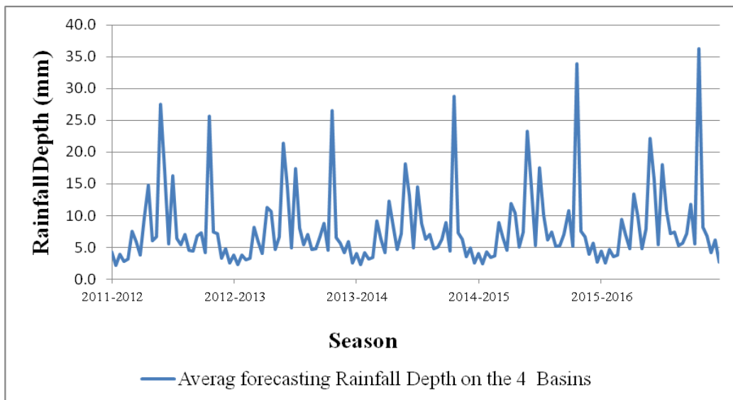
Figure 6: Average rainfall forecasting on the 4 basins for the up-coming 5 years (2012-2016)
