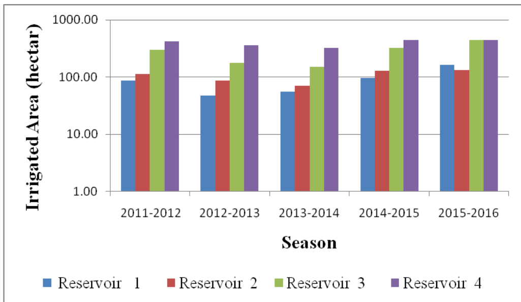
Figure 9: Irrigated area under combination both of supplemental irrigation and individual rainfall scenario of (S4, S5 and S6).
