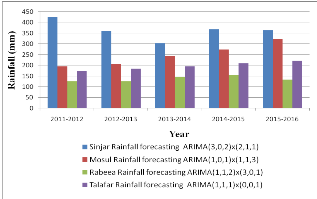
Figure 5 : Annual forecasting Rainfall for the four selected stations
