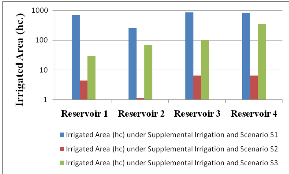
Figure 4: Resultant Irrigated Area by combination of Supplemental Irrigation and each of rainfall scenarios S1, S2, and S3
