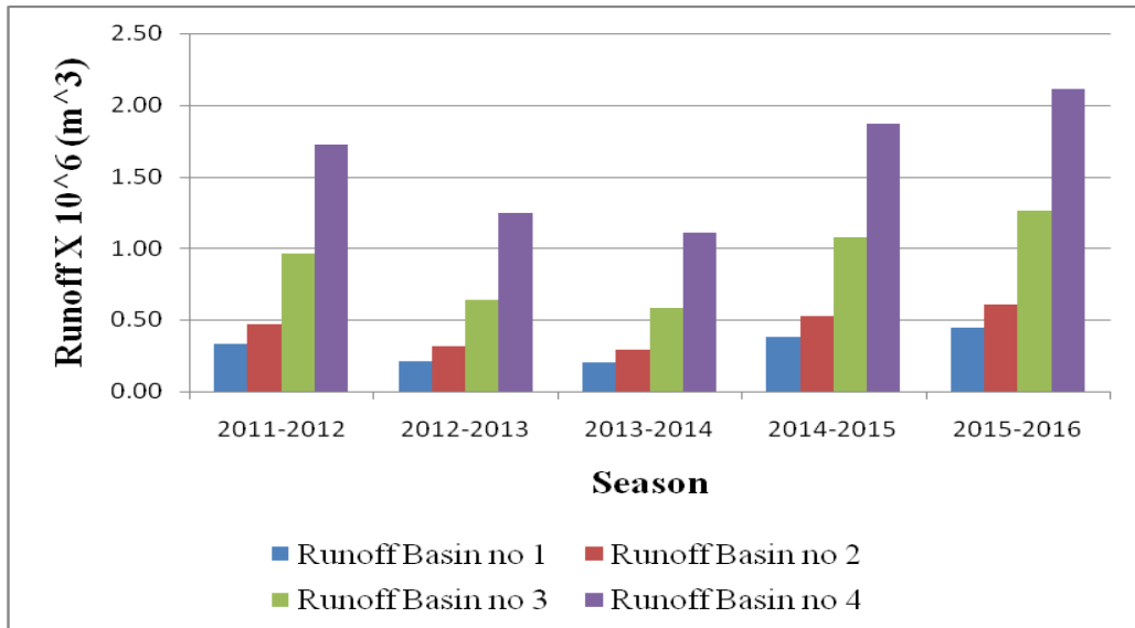
Figure 8: Runoff volumes for the up-coming 5 years (2012-2016).
